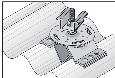
TopFix CorruBracket-AU fitted with S-5-PV Kit (purchased separately).
