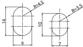
Mounting Hole
