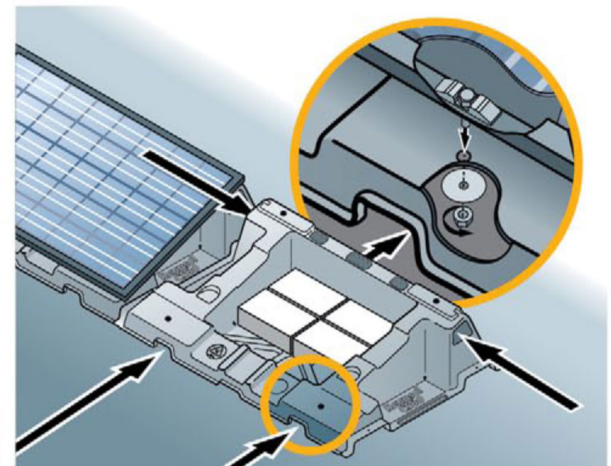
Fasten panel to Renusol CS60
