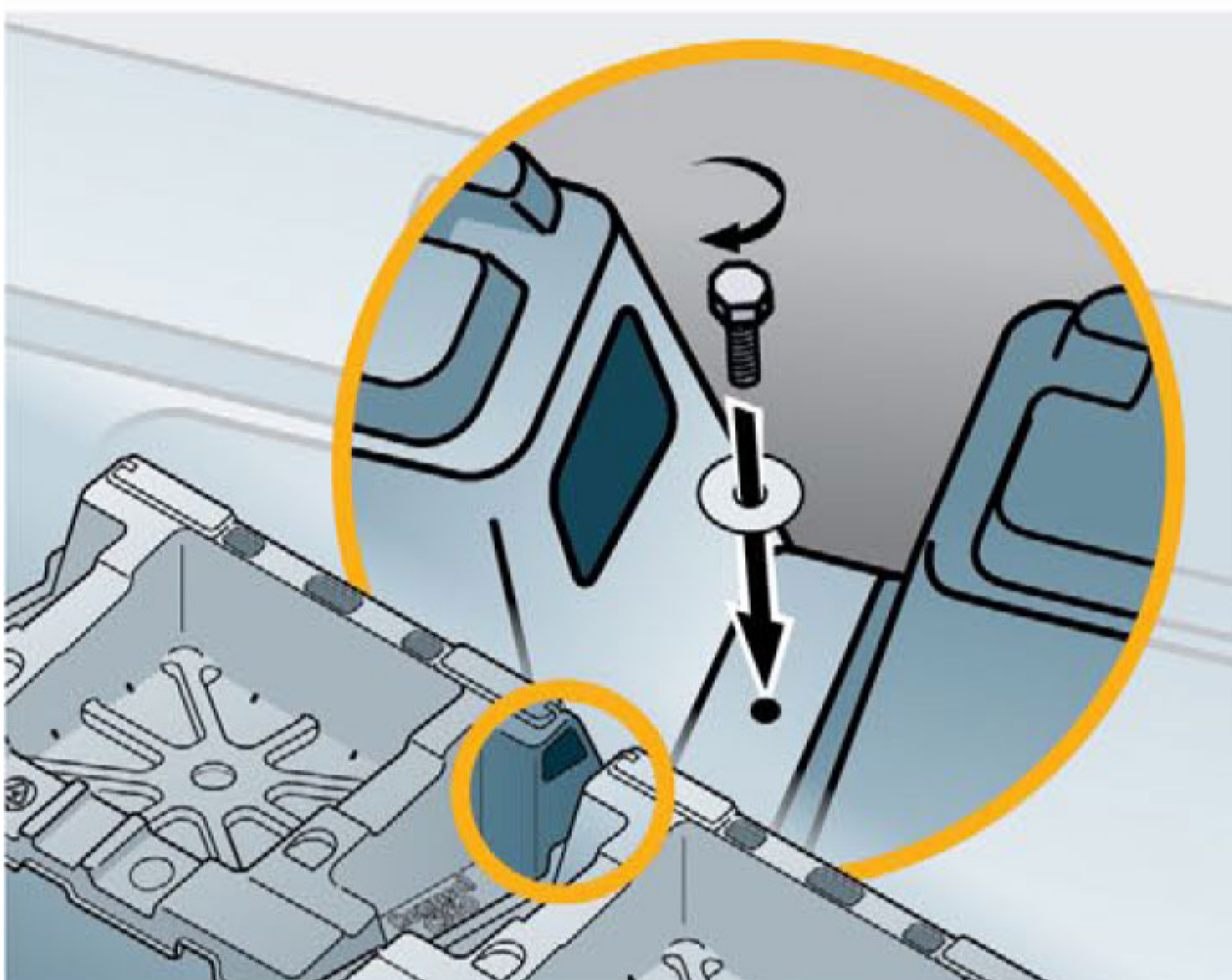
Fasten East-West, add ballast if needed
