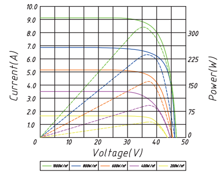
TP672P Pm(W)310
