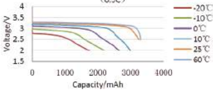
Discharge curves at different temperature (0.5C)
