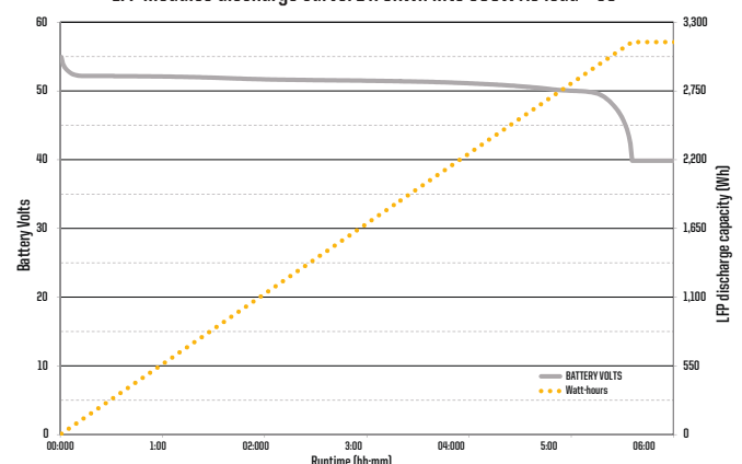
LFP modules discharge curve: 1 x 3kWh into 500W AC load = C6
