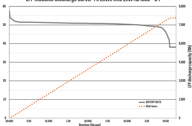
LFP modules discharge curve: 4 x 2kWh into 2kW AC load = C4
