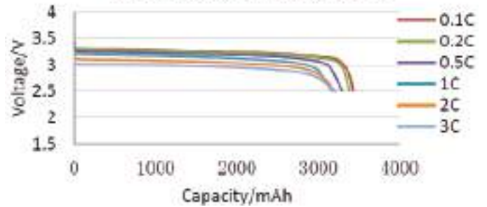
Discharge curves at different rates
